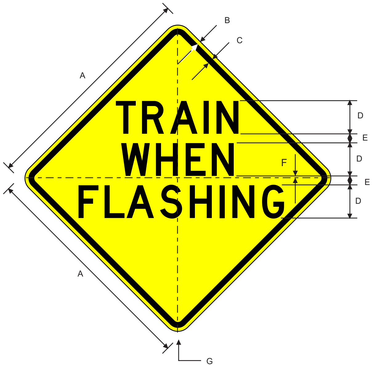
W10-4B TRAIN WHEN FLASHING
