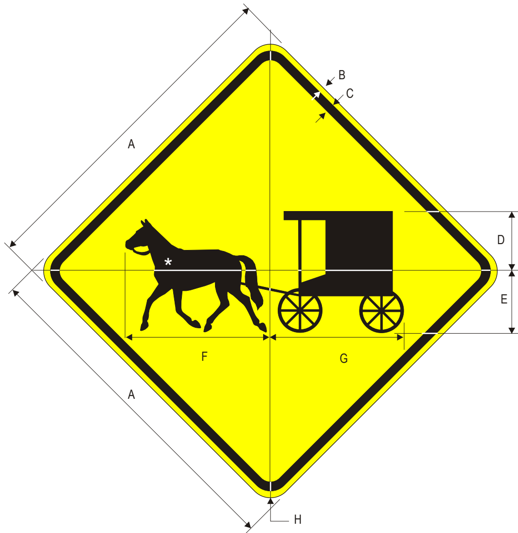
W11-14 Horse and Buggy Traffic (Symbol)
