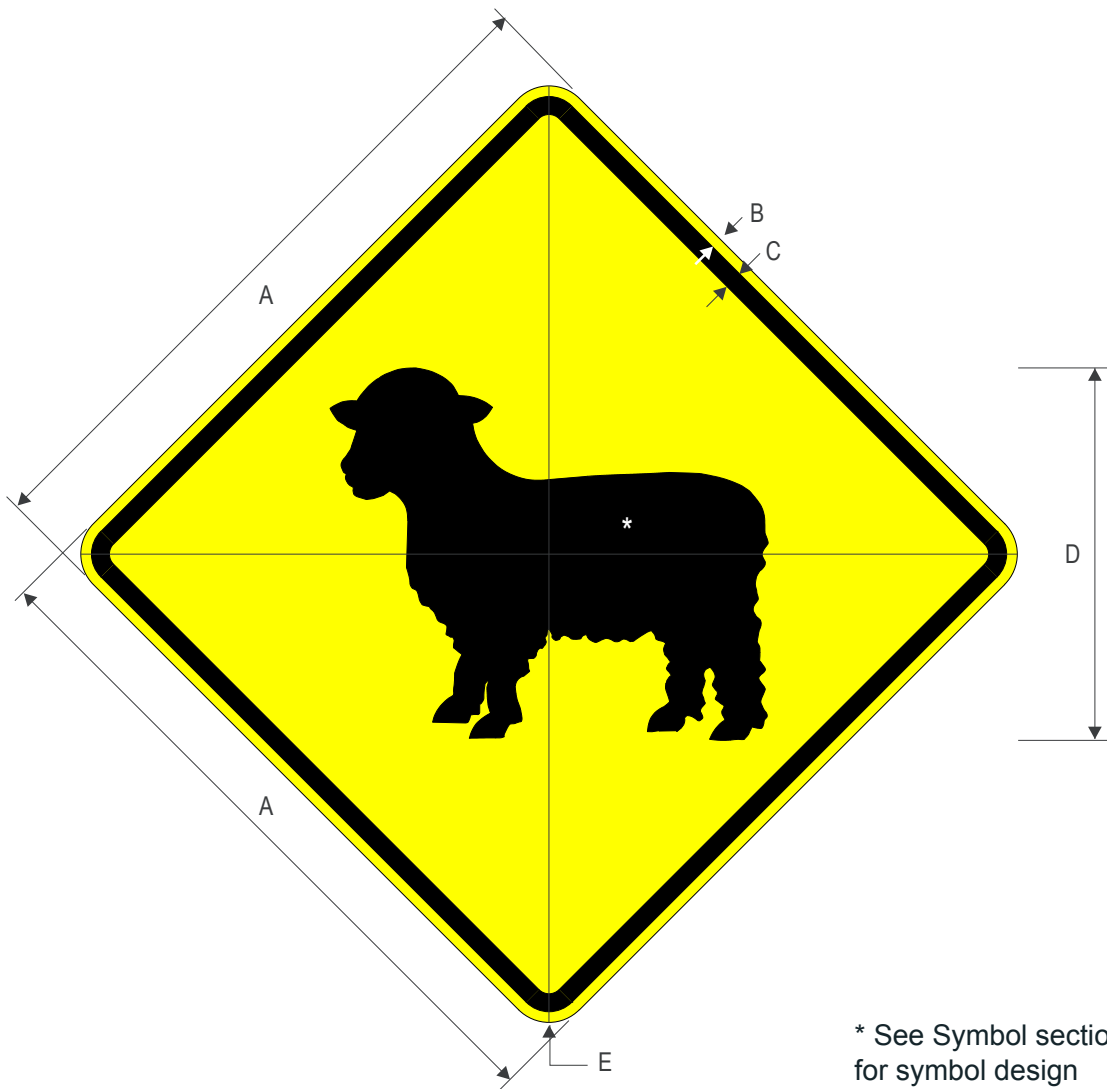
W11-17 (Sheep)
