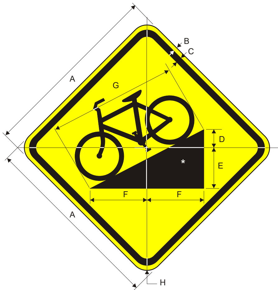
W7-5 Hill (Bike Symbol)
