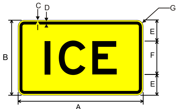
W8-5aP
