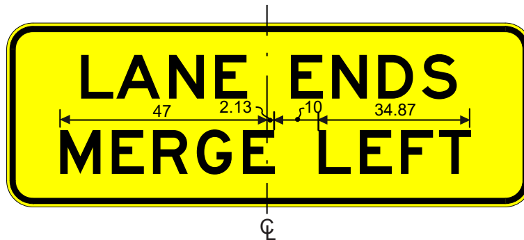
W9-5TL LANE ENDS MERGE LEFT
