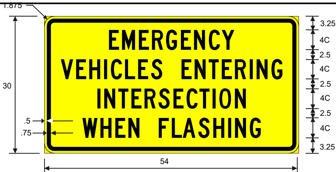
W11-12aT EMERGENCY VEHICLE ENTERING INTERSECTION WHEN FLASHING
