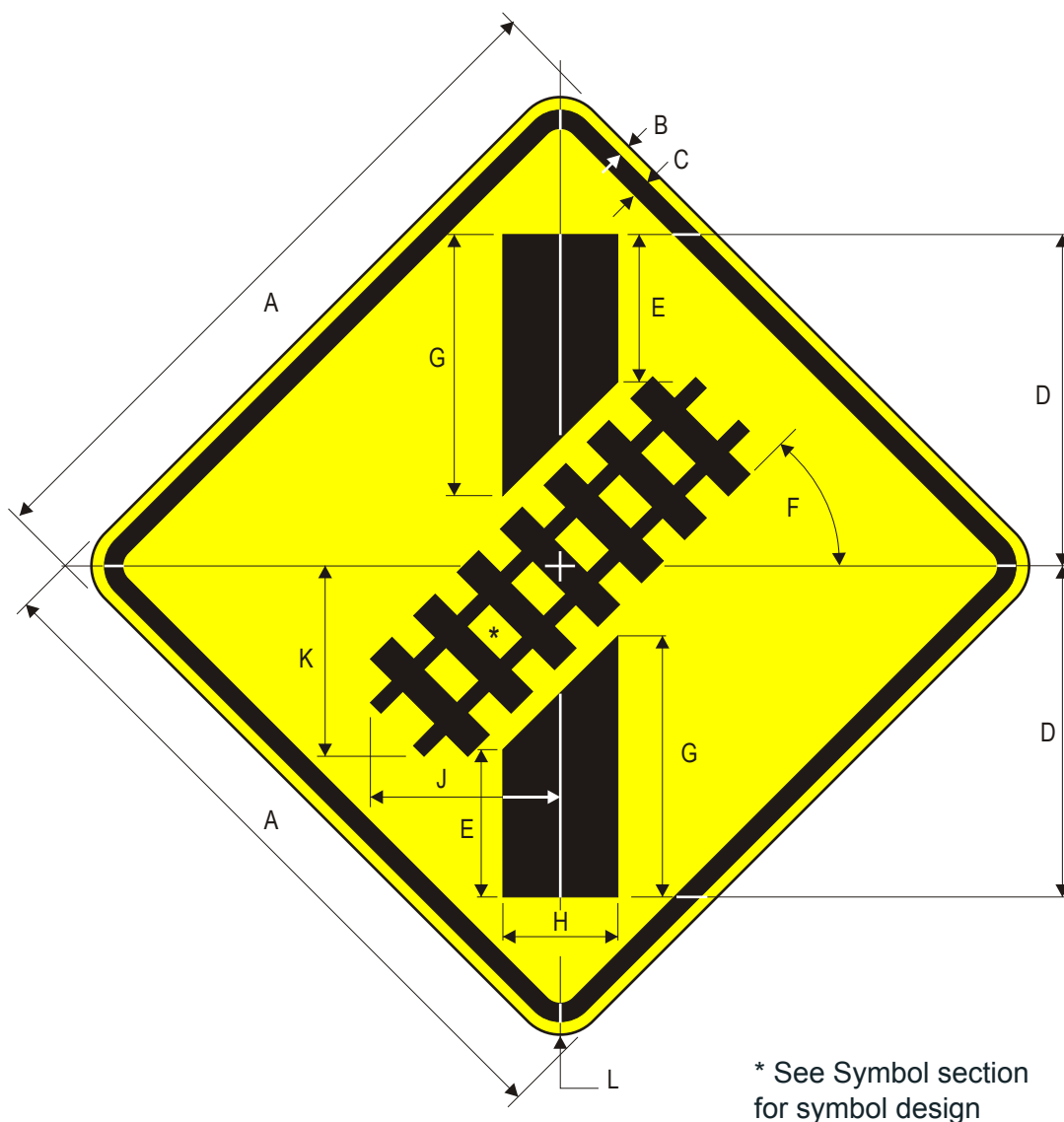
W10-12
