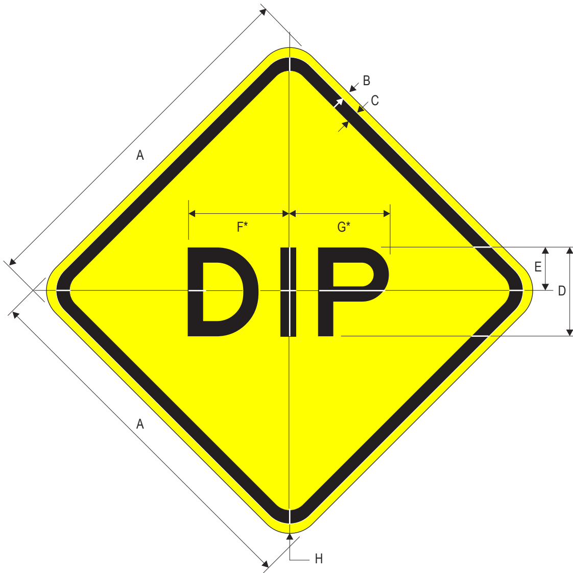
W8-2 DIP
