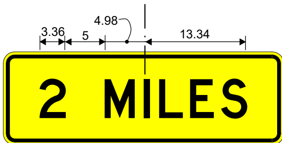
W16-3aTP (4)
