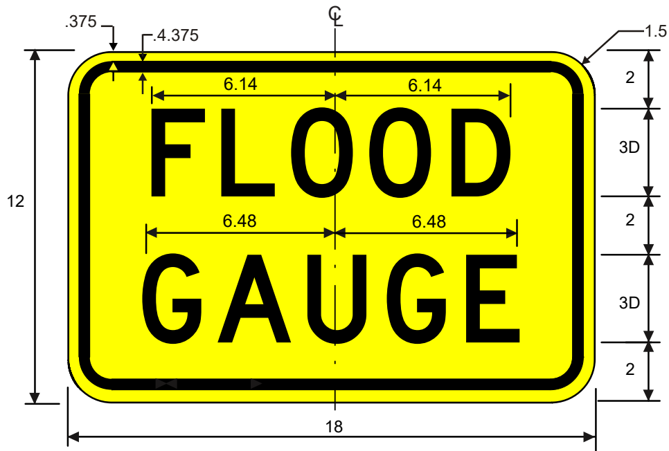
W8-19aTP FLOOD GAUGE (Plaque)
