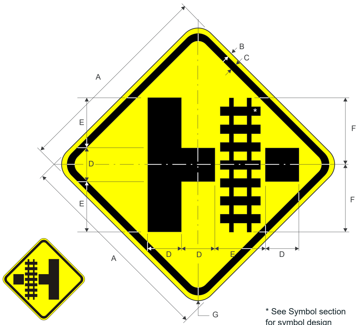
W10-3L
