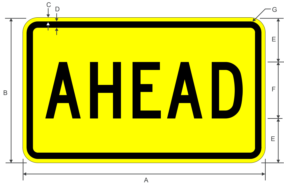
W16-9P AHEAD (Plaque)
