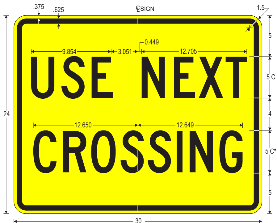
W10-14aP USE NEXT CROSSING * Reduce character spacing 20%.
