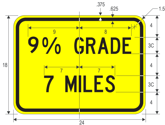
W7-3bP W7-3bP _ % X MILES (Plaque) COLORS: LEGEND - BLACK BACKGROUND - YELLOW
