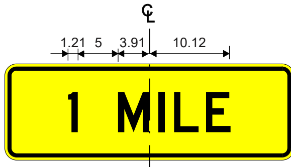
W16-3aTP (2)
