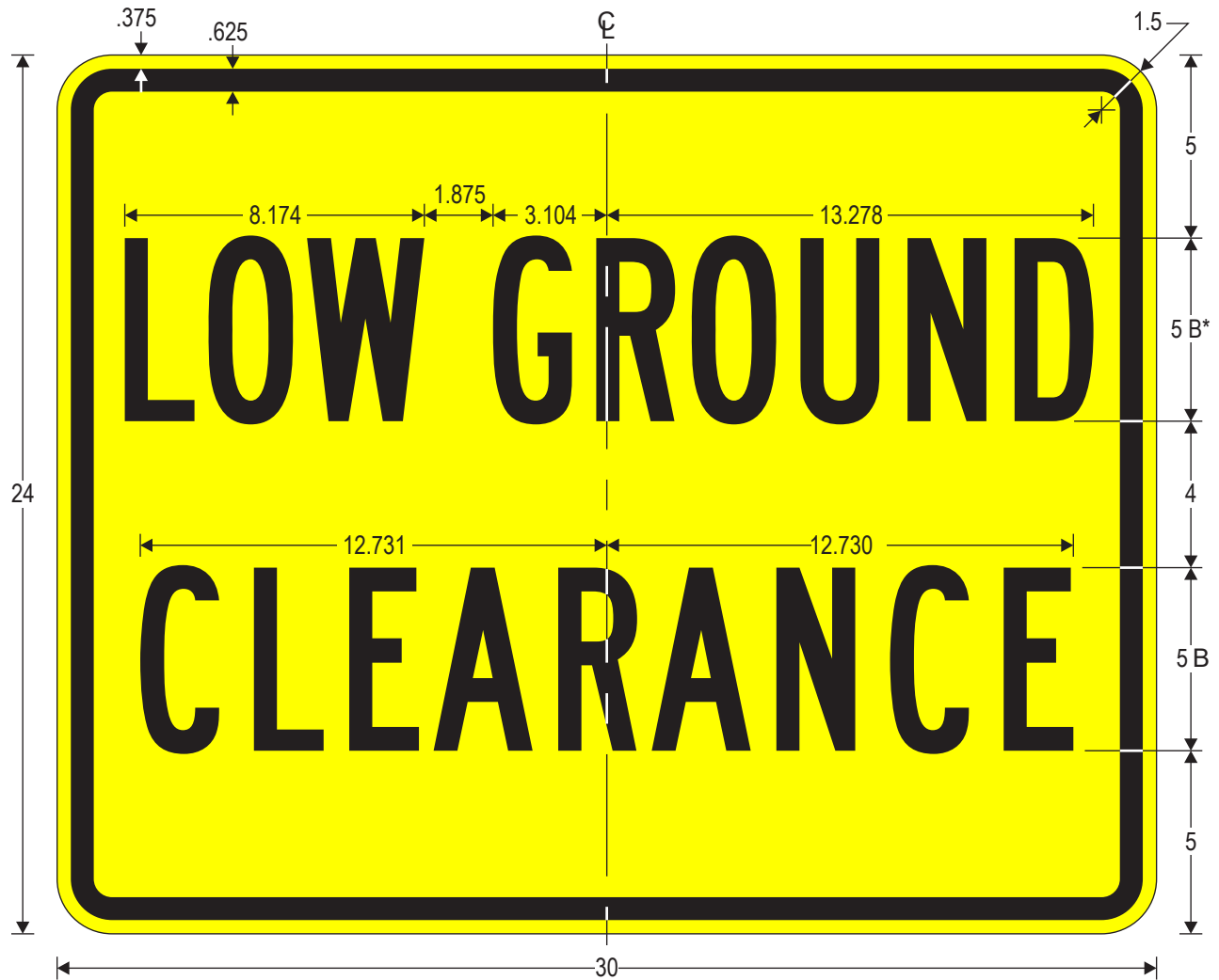
W10-5P LOW GROUND CLEARANCE (Plaque)
