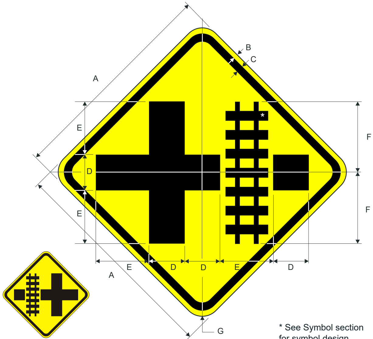
W10-2L
