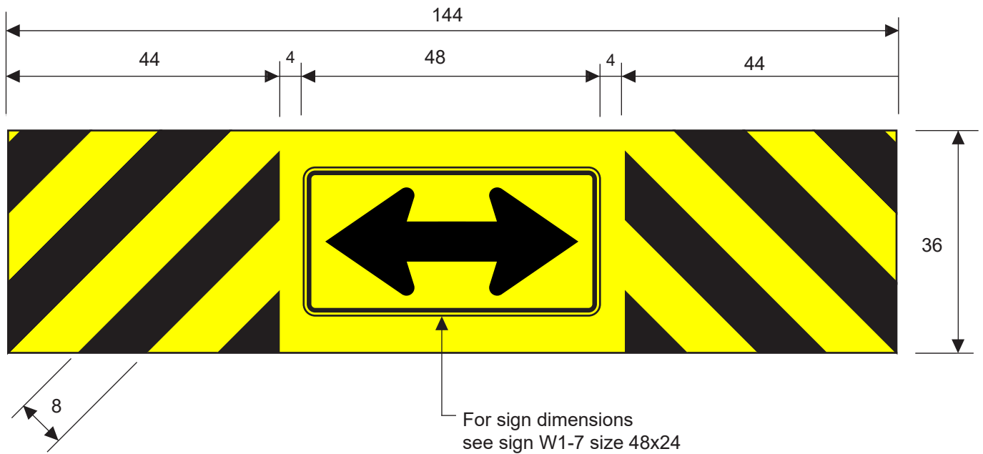
W1-7T Chevron/Two-Direction Large Arrow
