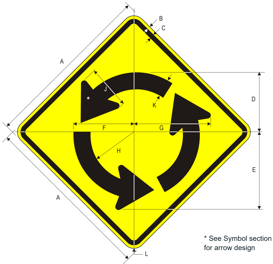
W2-6 Roundabout
