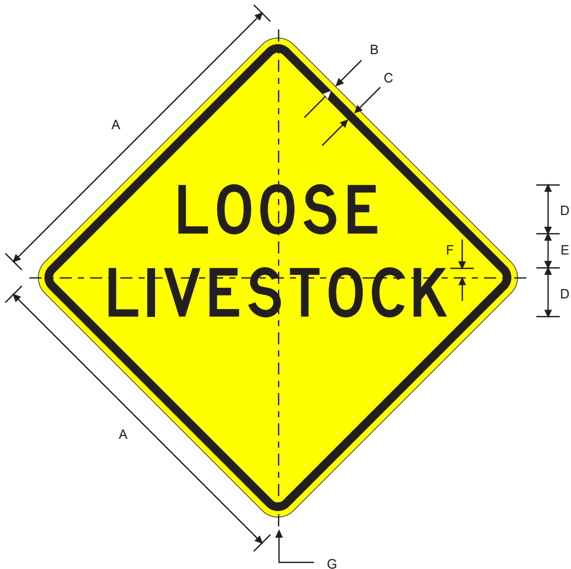
W17-3T LOOSE LIVESTOCK
