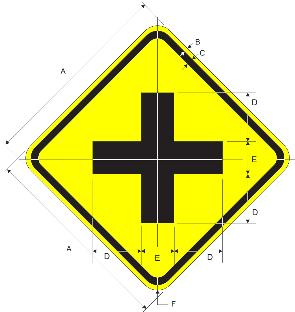
W2-1 Crossroad
