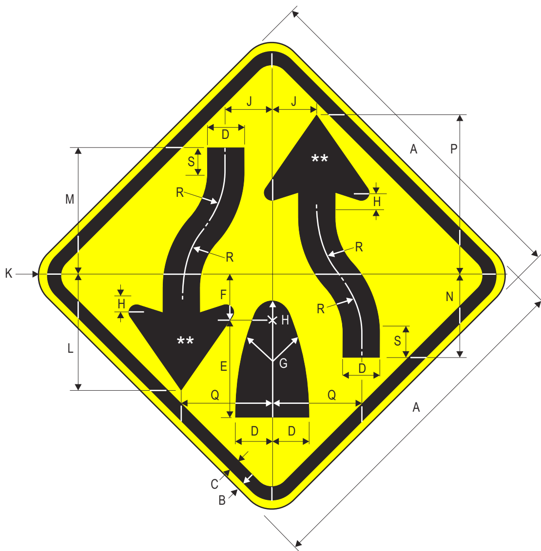
W6-2 Divided Highway Ends (Symbol)
