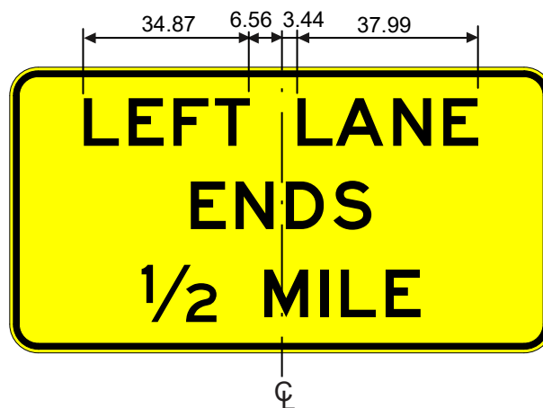
W9-4TL LEFT LANE ENDS 1/2 MILE
