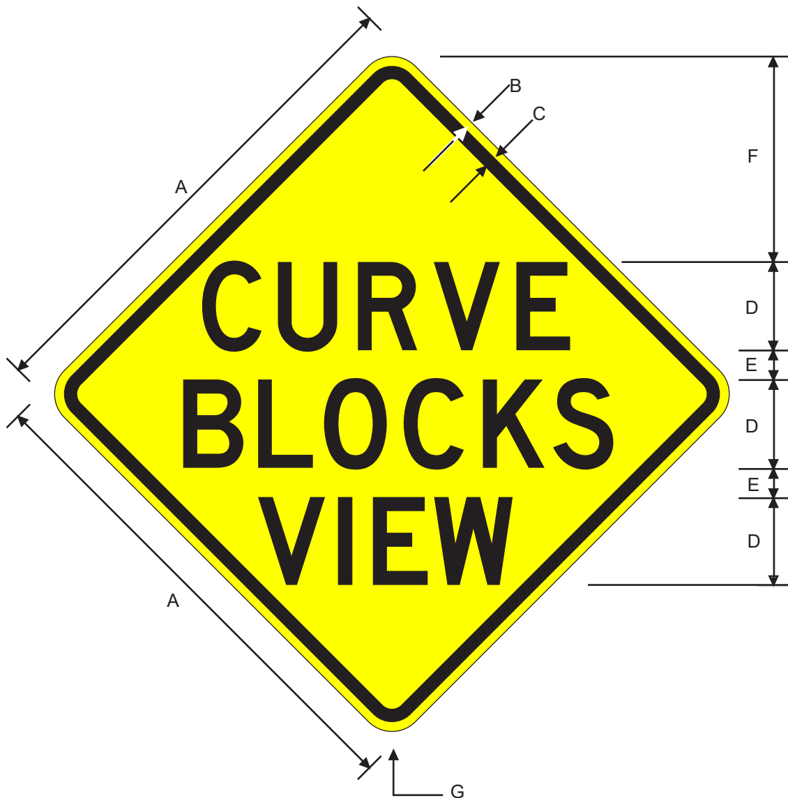
W1-11T CURVE BLOCKS VIEW
