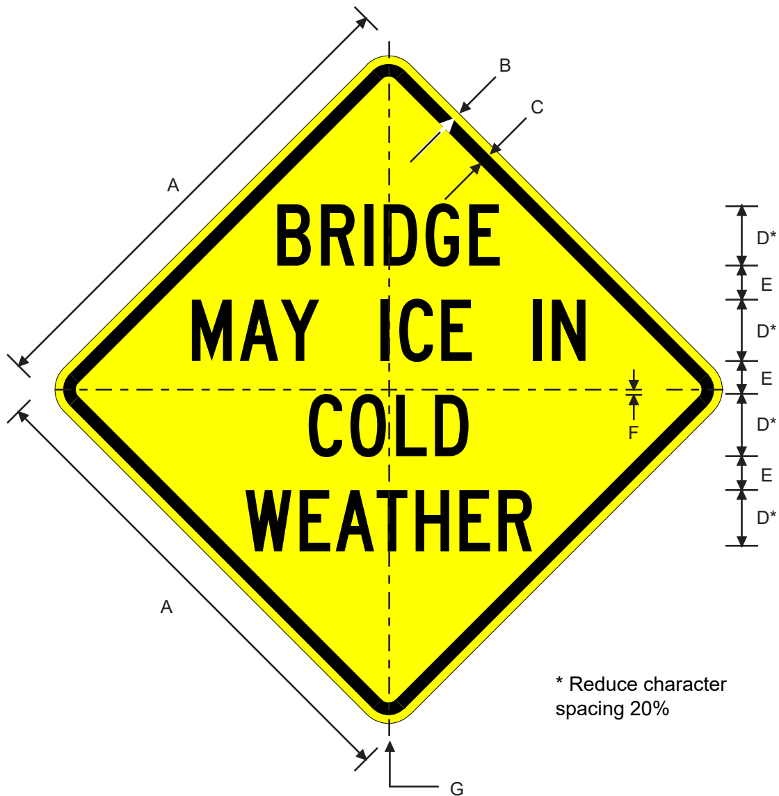
W8-13aT BRIDGE MAY ICE IN COLD WEATHER
