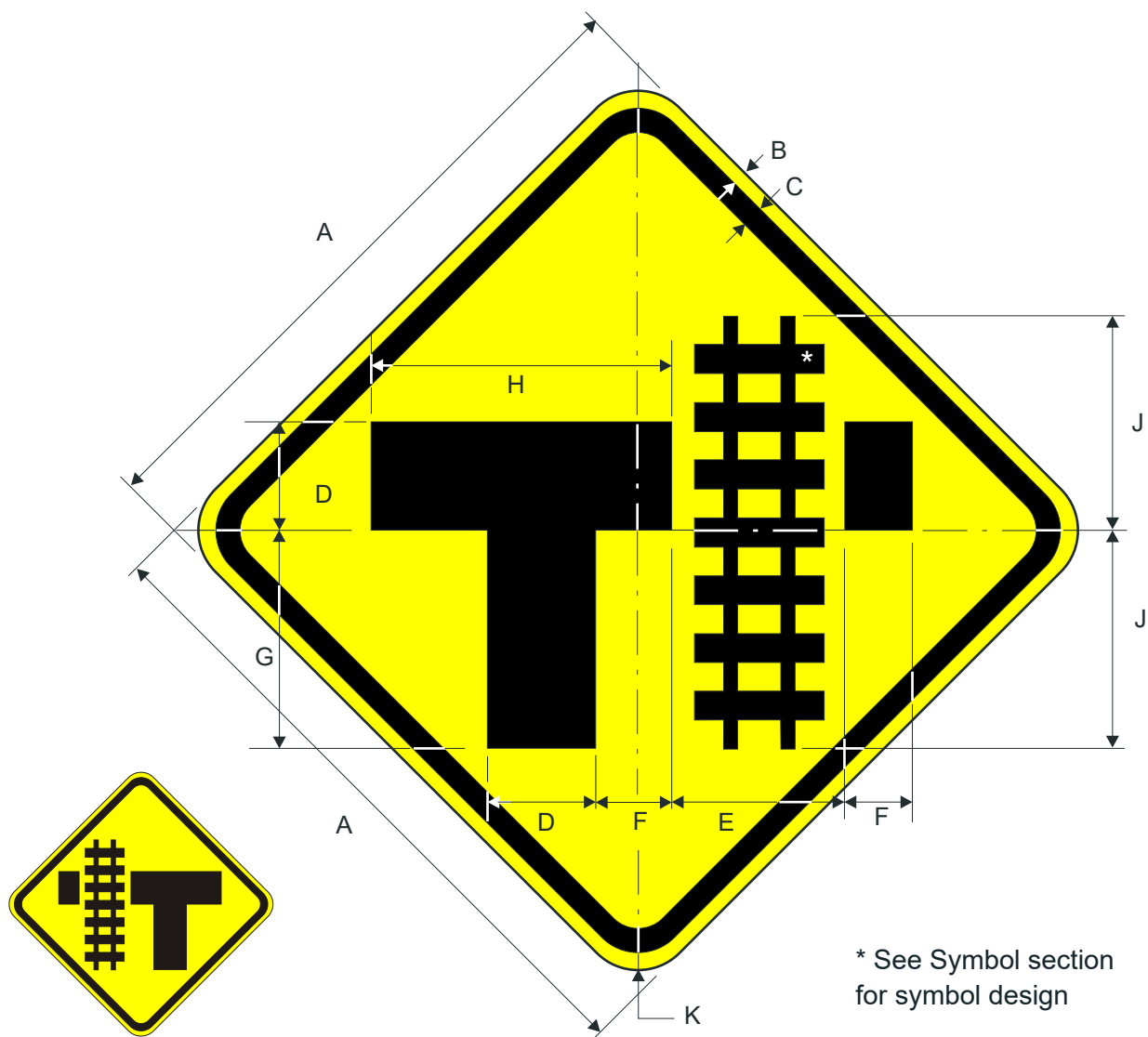
W10-4L
