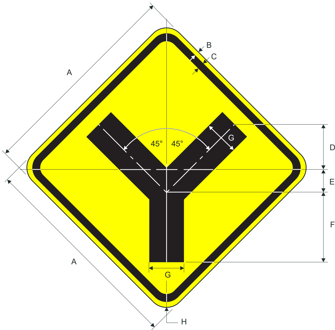
W2-5 "Y" Intersection
