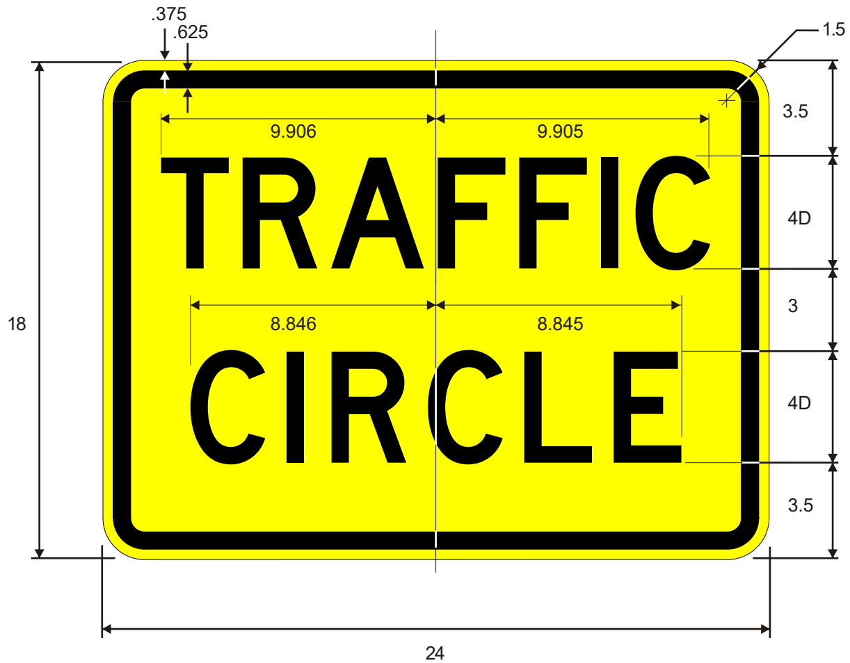
W16-12P TRAFFIC CIRCLE (Plaque)
