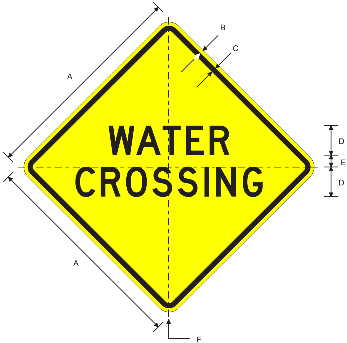
W8-18aT WATER CROSSING
