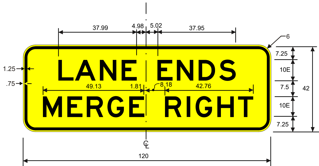
W9-5TR LANE ENDS MERGE RIGHT
