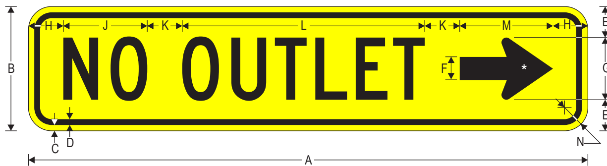
W14-2aR NO OUTLET (Arrow)
