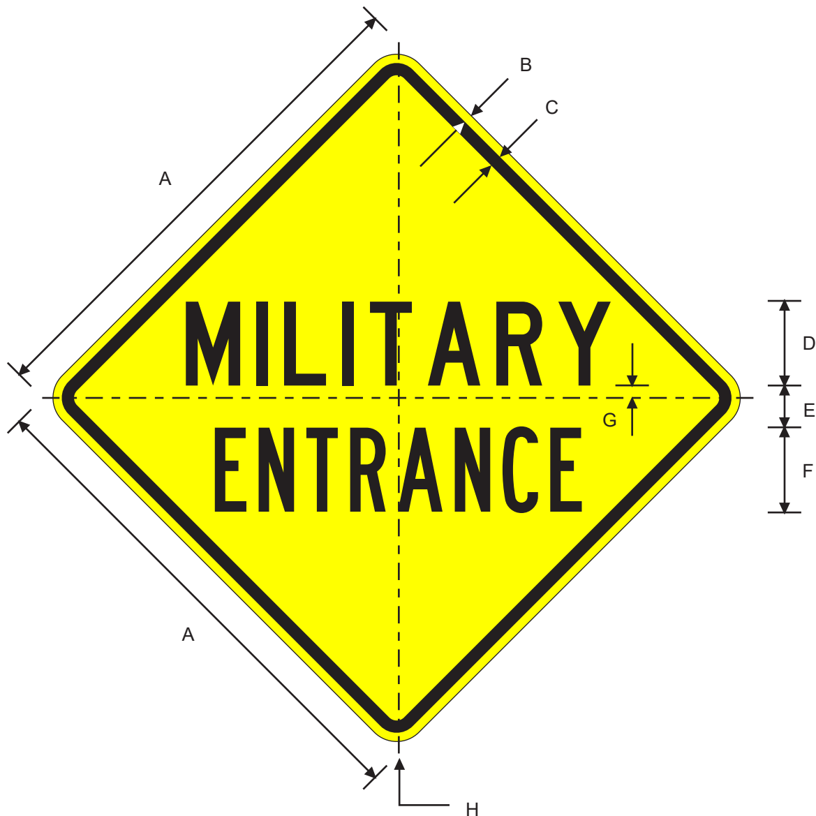
W17-6T MILITARY ENTRANCE
