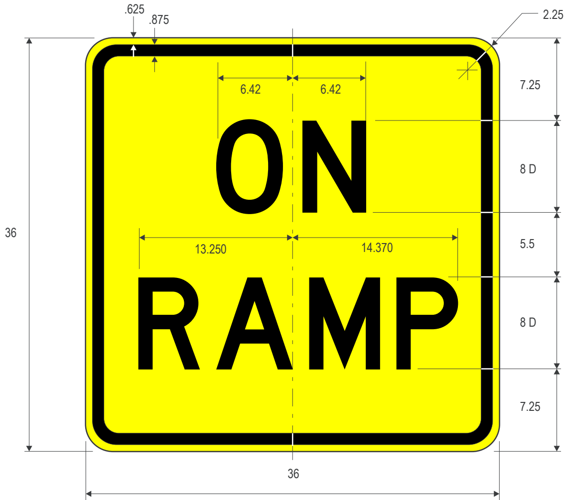
W13-4P ON RAMP
