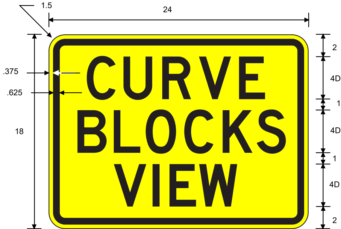
W1-11TP CURVE BLOCKS VIEW (Plaque)
