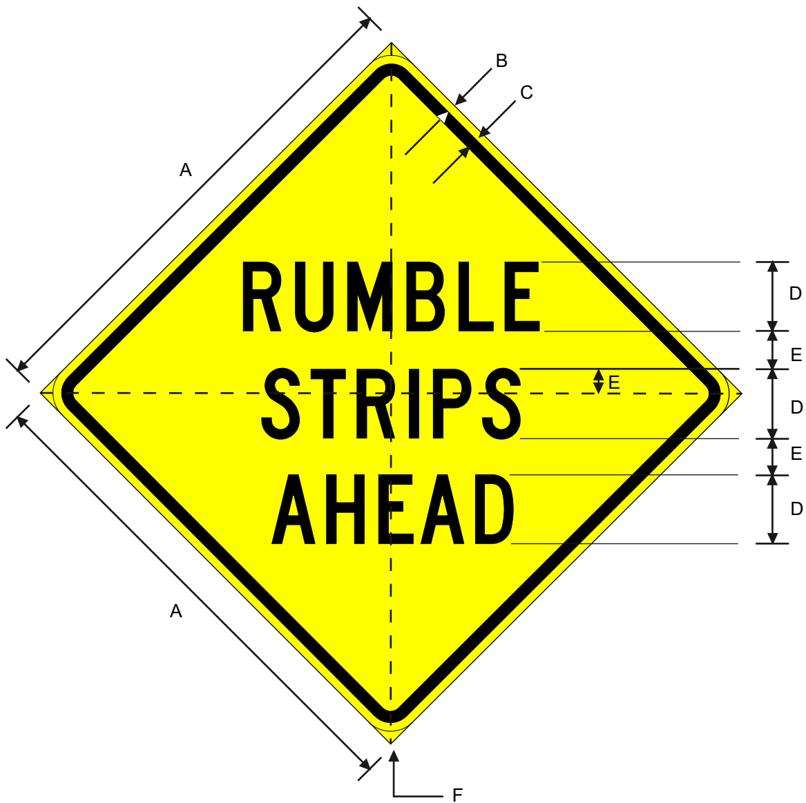
W17-2T RUMBLE STRIPS AHEAD
