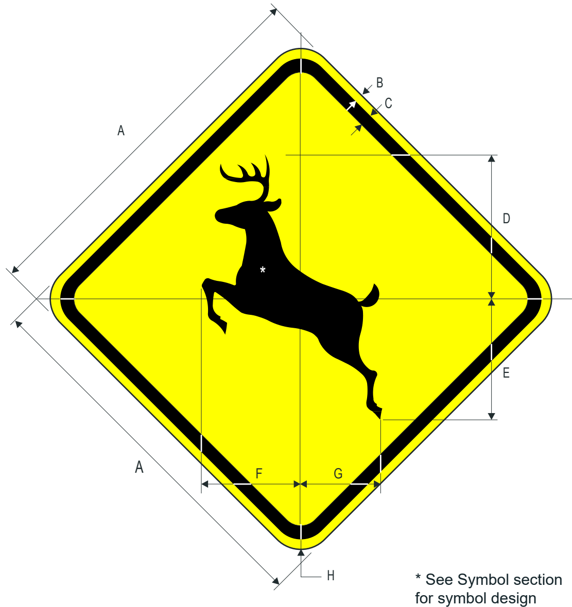
W11-3 Deer Crossing (Symbol)
