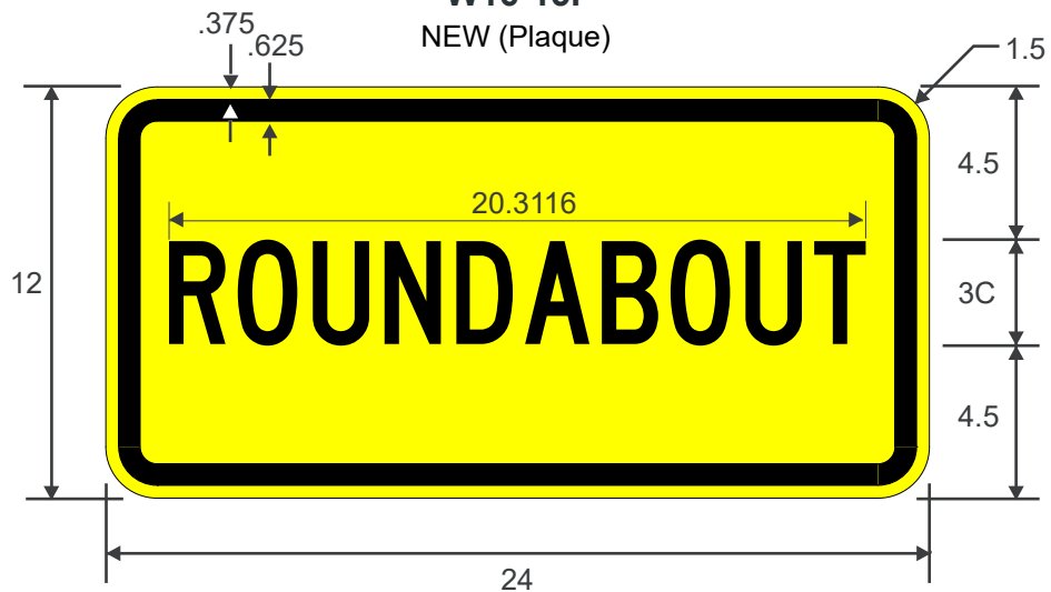
W16-17P ROUNDAABOUT (Plaque)
