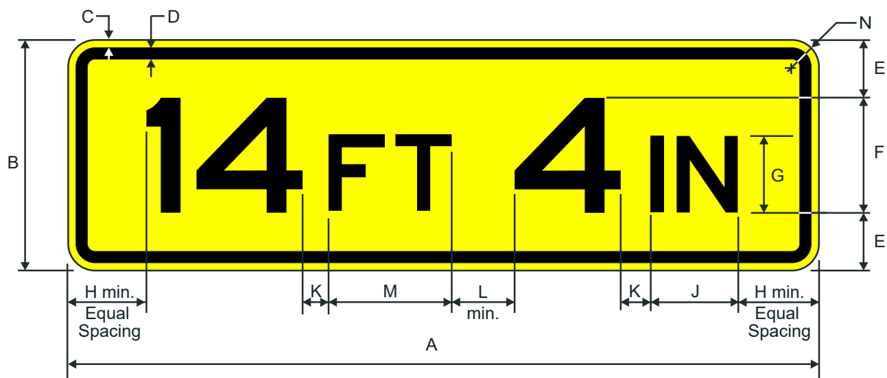
W12-2a __FT __IN (Low Clearance)
