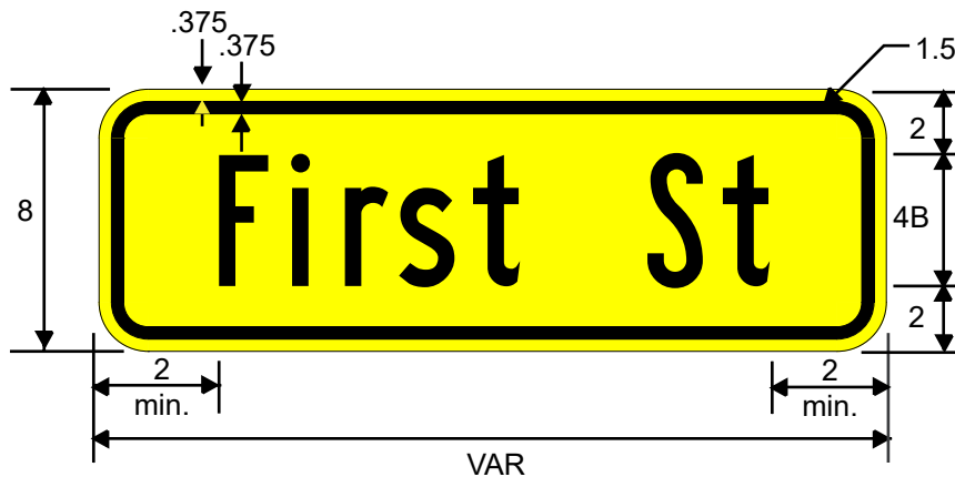
W16-8P Advance Street Name (Plaque)
