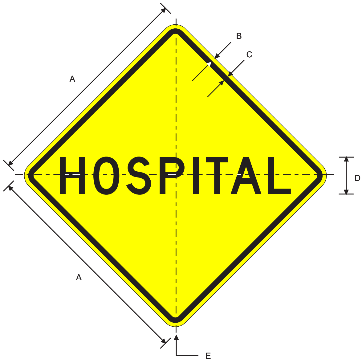
W17-5T HOSPITAL
