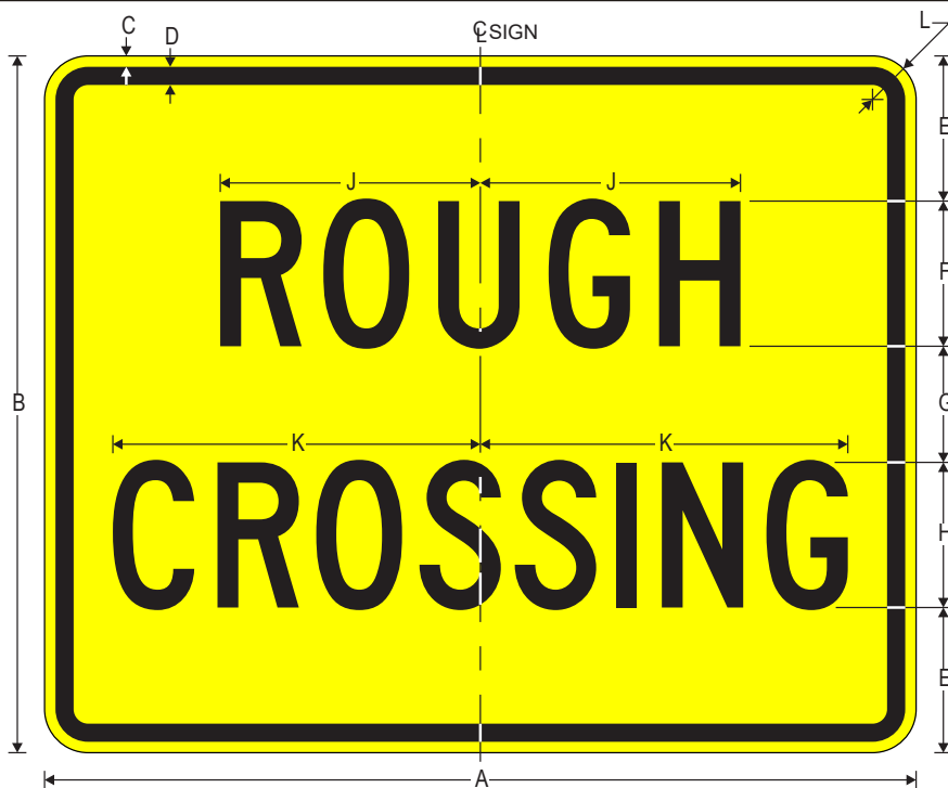
W10-15P ROUGH CROSSING * Reduce character spacing 20%.
