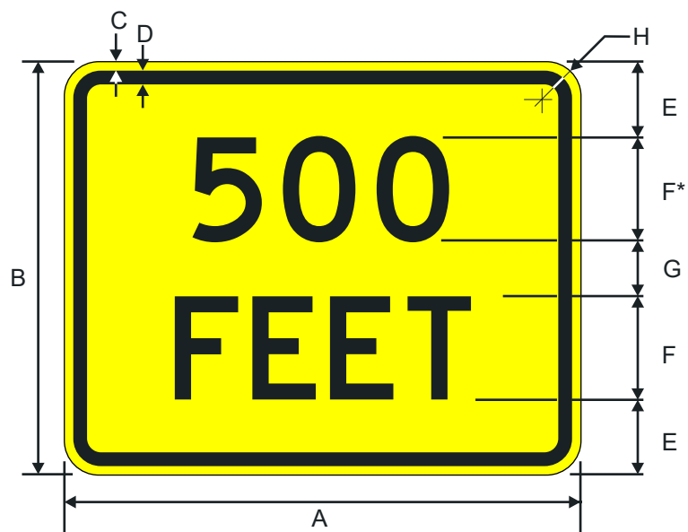
W16-2P Distance Plaque (2 lines)
