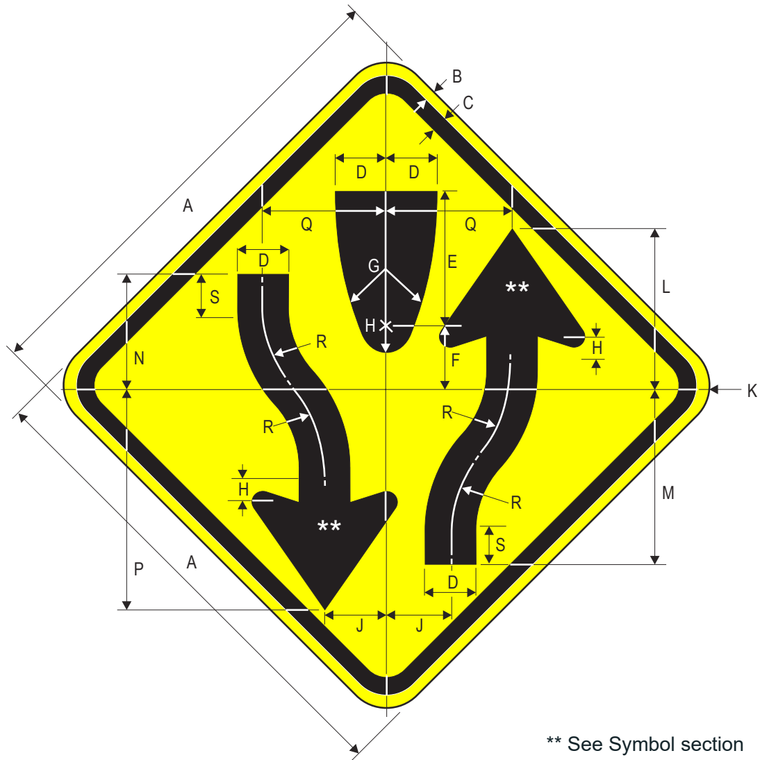
W6-1 Divided Highway Begins (Symbol)
